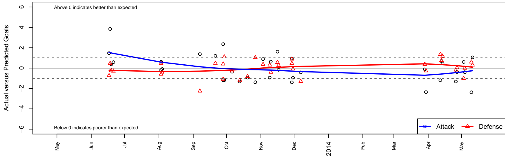
San Diego Surf SC Academy ECNL G99 Dots are actual minus expected GF (blue circles) and GA (red triangles). Blue line is smoothed change in attack strength. Red is smoothed change in defense strength.
